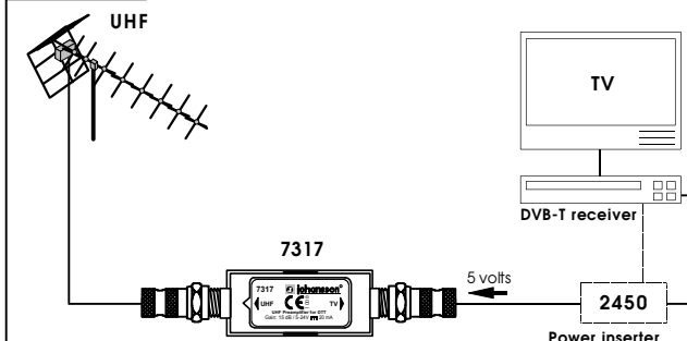
Fig. 1 The preamplifier is powered by the DVB-T receiver
