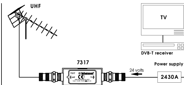
Fig. 2 The preamplifier is powered with an external power supply
